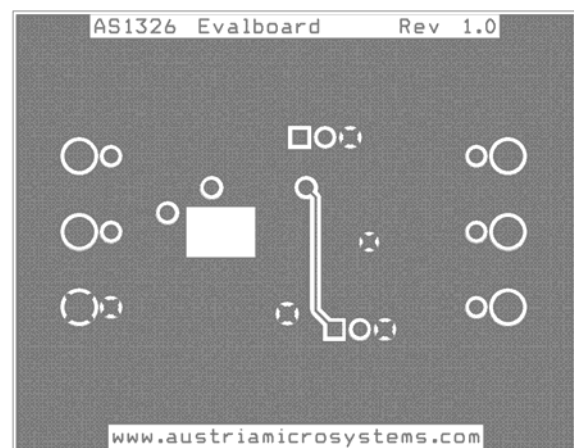
Figure 5: Bottom view
